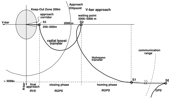
Figure 5.25. Approach strategy to –V-bar docking port (example 1).
