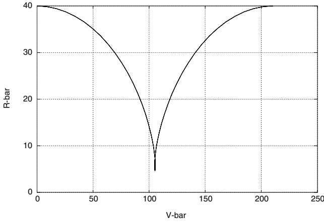
Figure 3.16. Example: impulse of \Delta V_x = 0.01 m/s, starting 40 m below target orbit.
